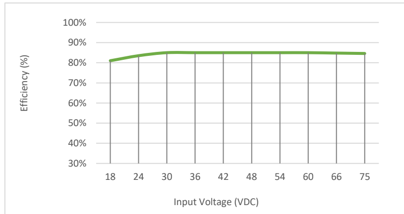
SDU06P4815D, with full Load
