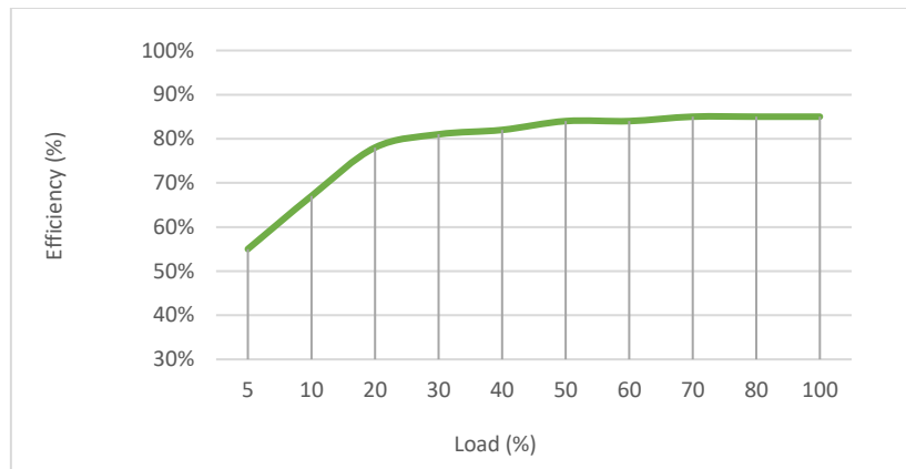
SDU06P4815D, with nominal input voltage
