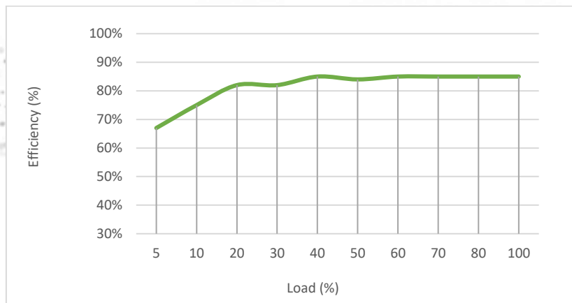
SDU06P2405, with nominal input voltage
